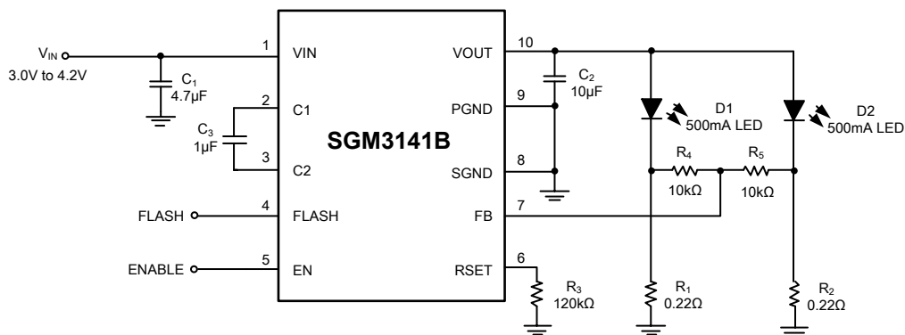
Figure 3. Two Flash LED Drive
