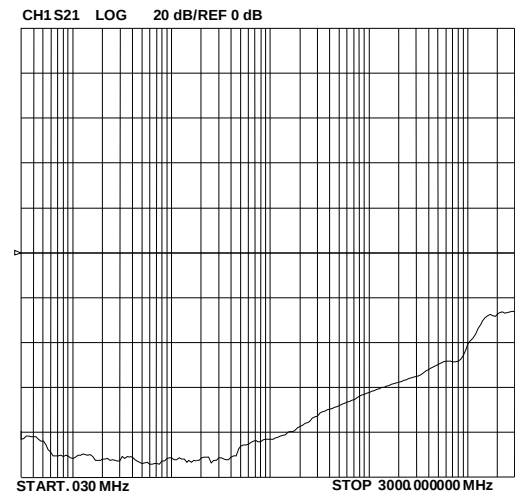
Analog Crosstalk
