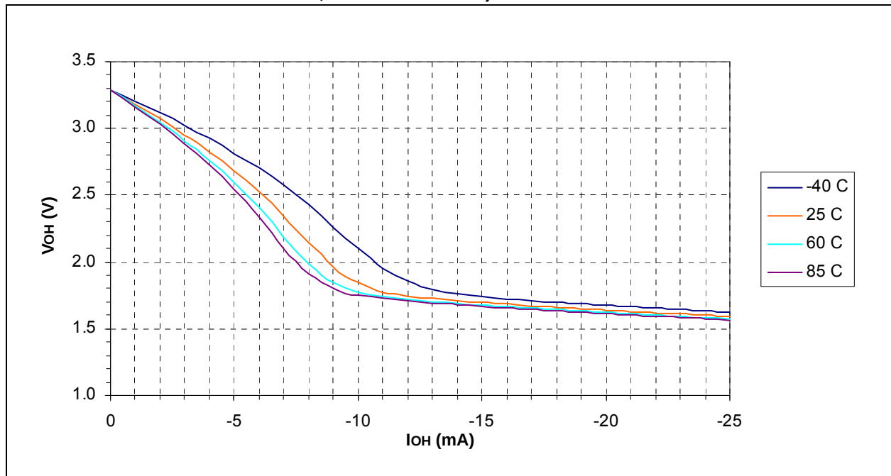
FIGURE 30-25: TYPICAL V_{OH} vs. I_{OH} (GENERAL PURPOSE I/O, AS A FUNCTION OF TEMPERATURE, 2.0V \leq V_{DD} \leq 5.5V )
