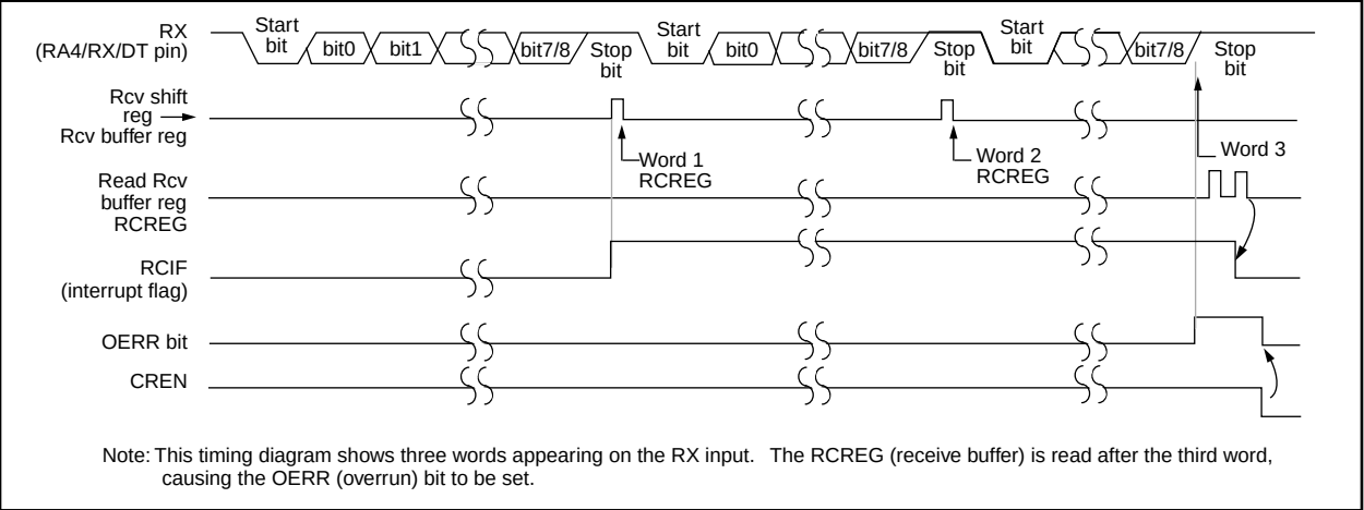
FIGURE 13-8: ASYNCHRONOUS RECEPTION
