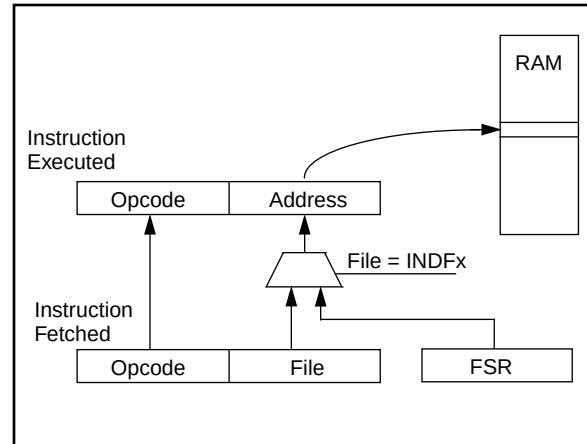
FIGURE 6-10: INDIRECT ADDRESSING
