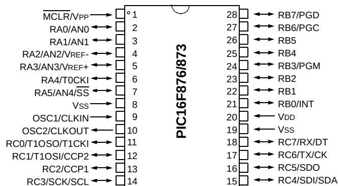
PDIP, SOIC
