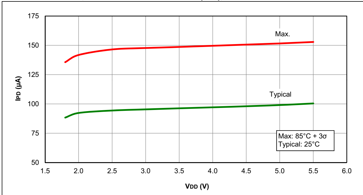
FIGURE 23-19: I_{PD} , FIXED VOLTAGE REFERENCE (FVR), PIC16F753 ONLY
