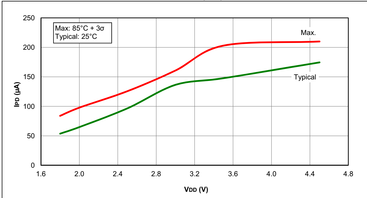
FIGURE 23-18: I_{PD} , FIXED VOLTAGE REFERENCE (FVR), PIC16HV753 ONLY
