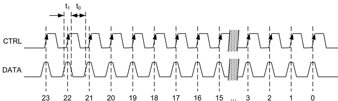
FIGURE 9-4: RECOVERY SEQUENCE TIMING
