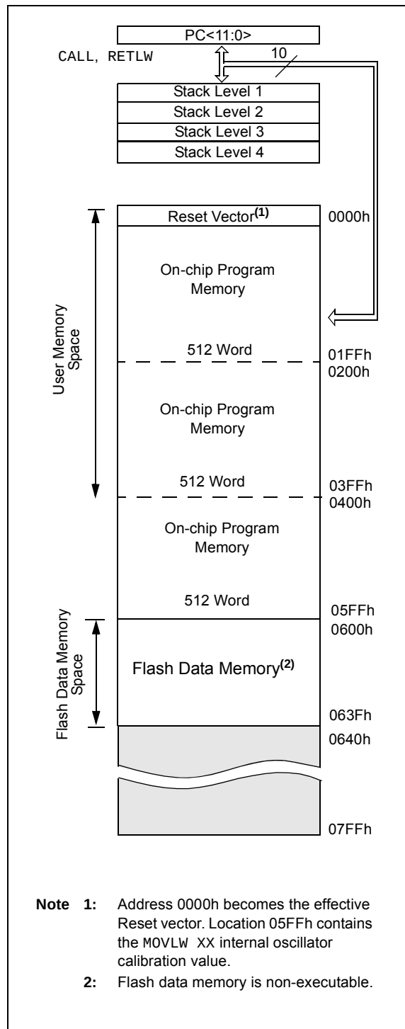
FIGURE 4-1: MEMORY MAP
