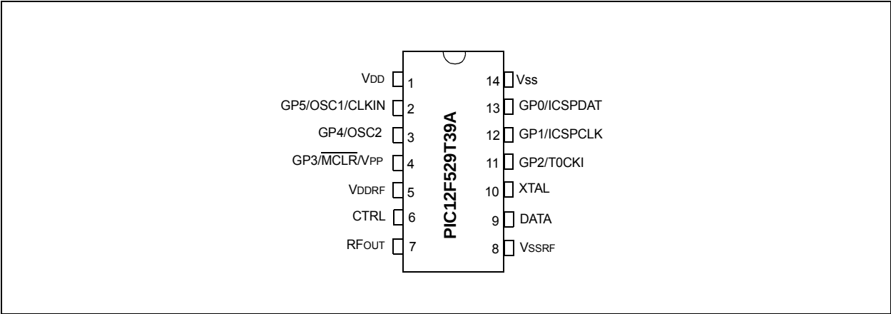
FIGURE 1: 14-PIN TSSOP
