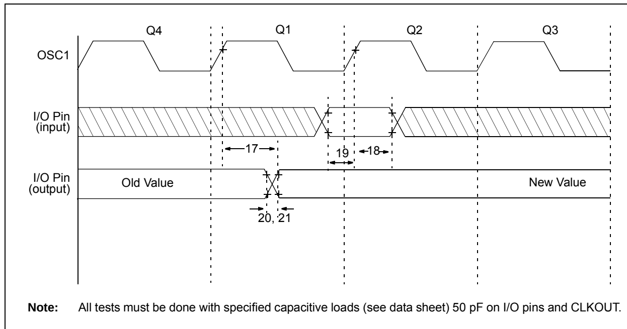
FIGURE 12-5: I/O TIMING
