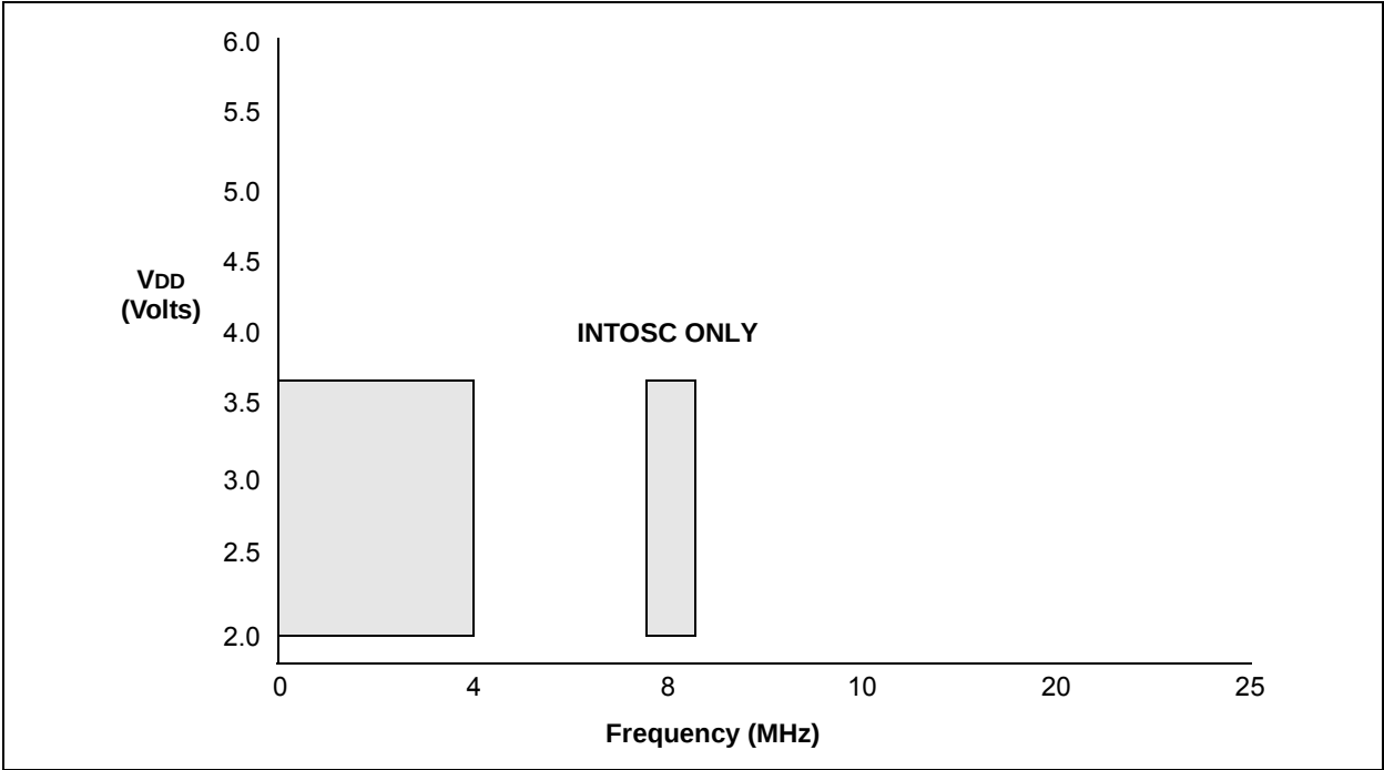
FIGURE 12-1: PIC12F529T39A VOLTAGE-FREQUENCY GRAPH, -40°C ≤ TA ≤ +85°C
