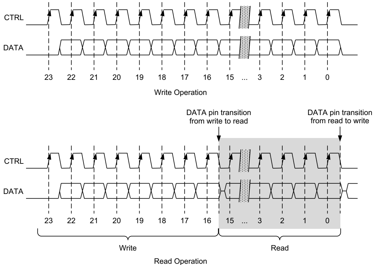
FIGURE 9-3: REGISTER WRITE AND READ OPERATIONS
