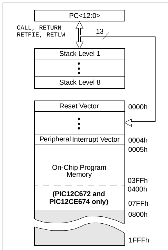
FIGURE 4-1: PIC12C67X PROGRAM MEMORY MAP AND STACK
