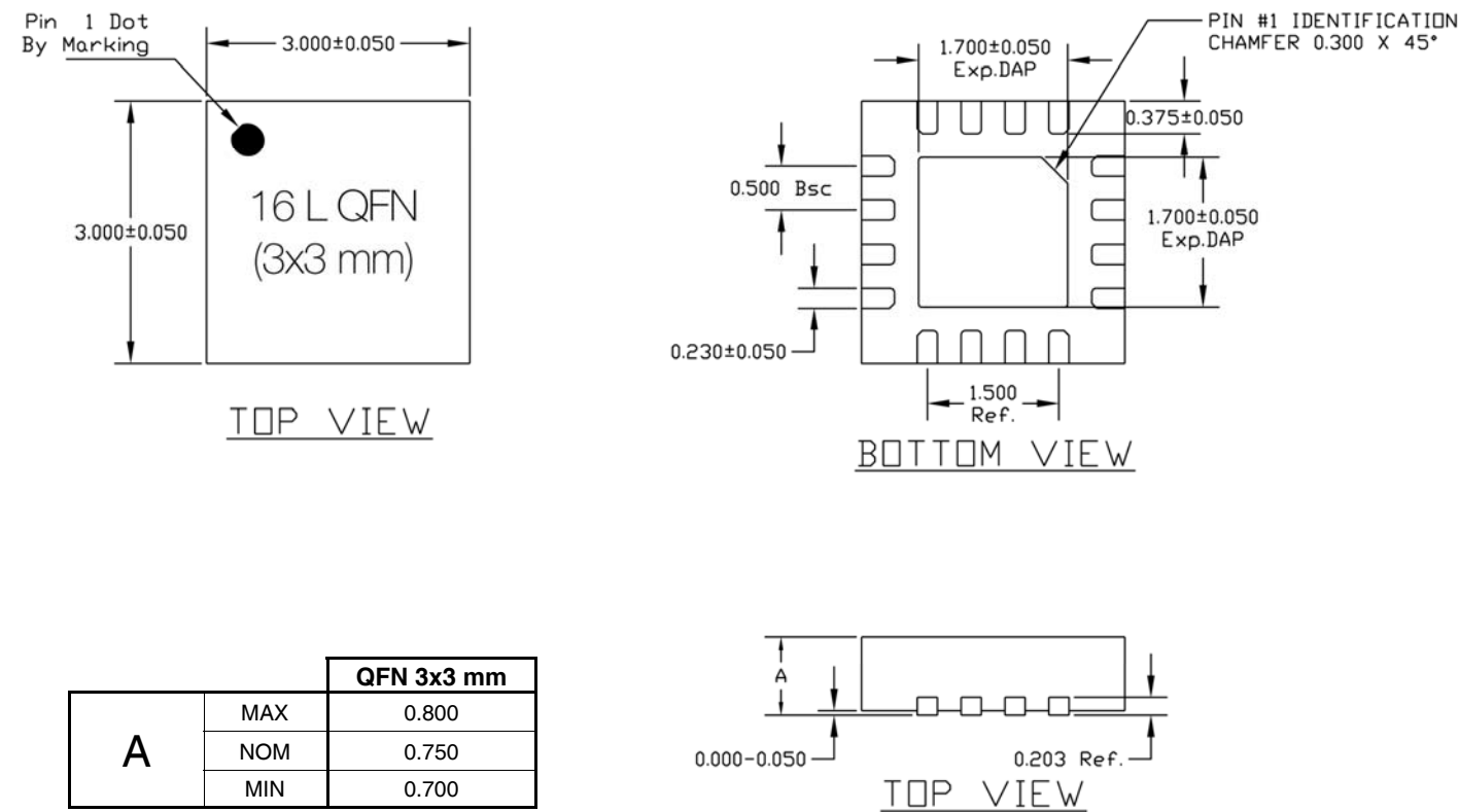
Figure 12. Package Drawing
