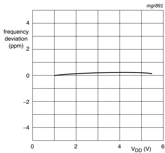
Fig 26. Frequency deviation as a function of supply voltage V_{DD}
