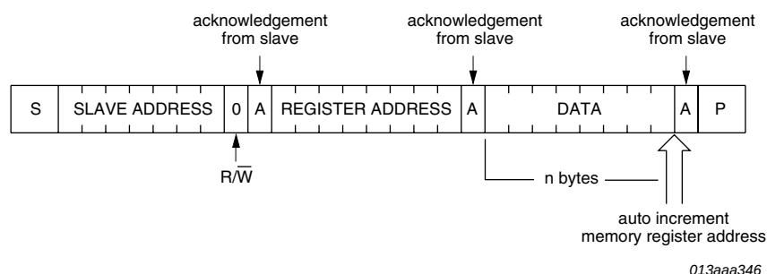
Fig 19. Master transmits to slave receiver (WRITE mode)
