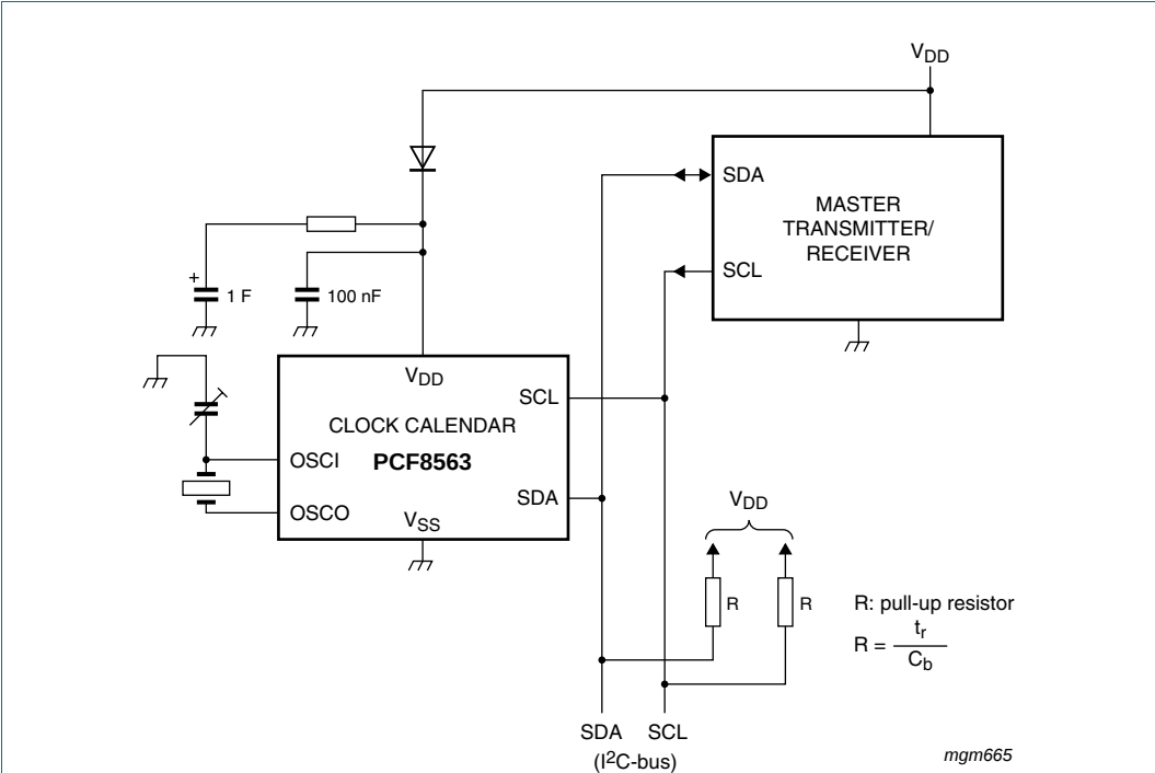
Fig 28. Application diagram
