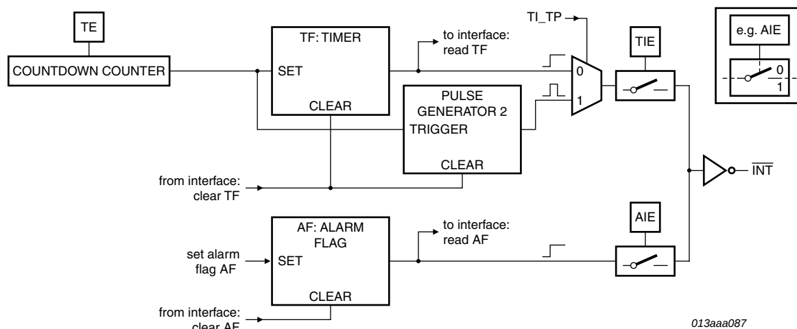
Fig 6. Interrupt scheme
