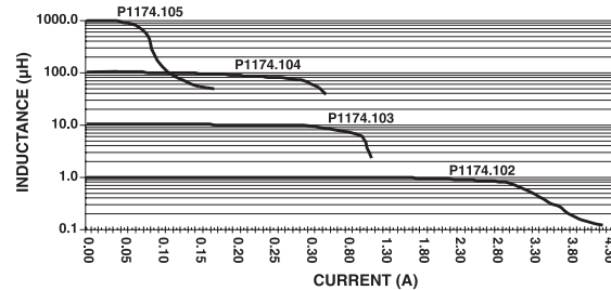
TYPICAL INDUCTANCE VS. DC BIAS
