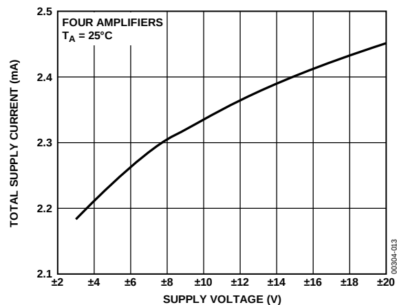
Figure 13. Total Supply Current vs. Supply Voltage
