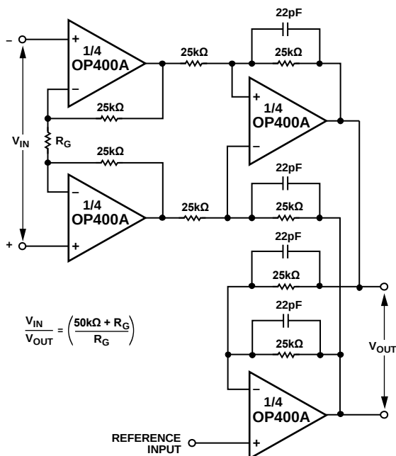
Figure 33. Differential Output Instrumentation Amplifier
