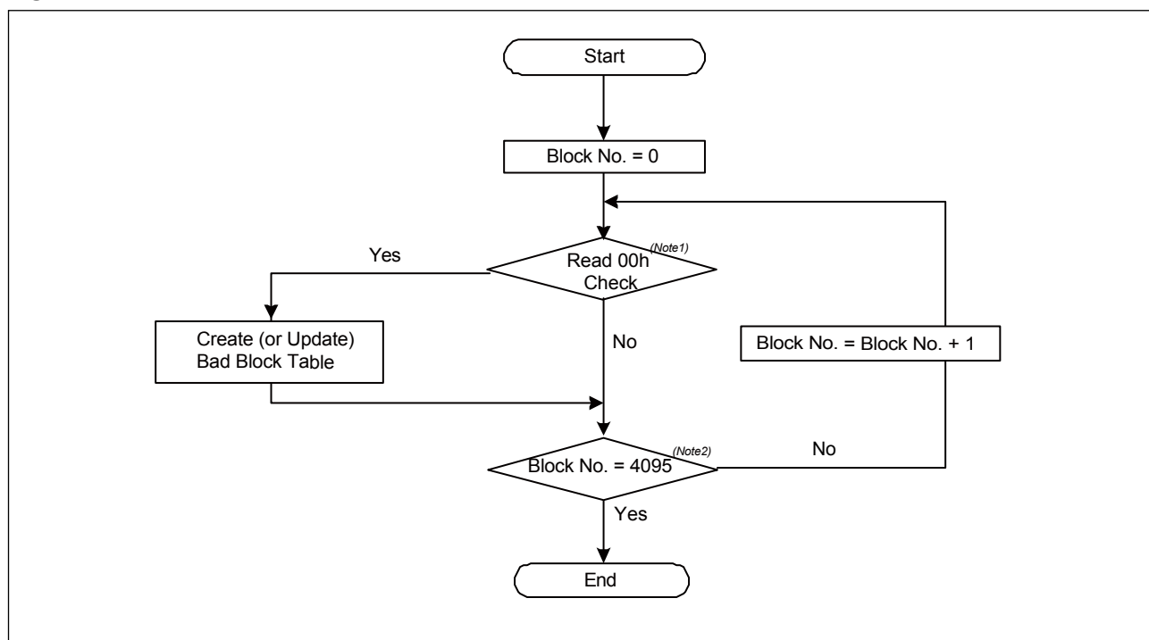
Figure 42. Bad Block Test Flow
