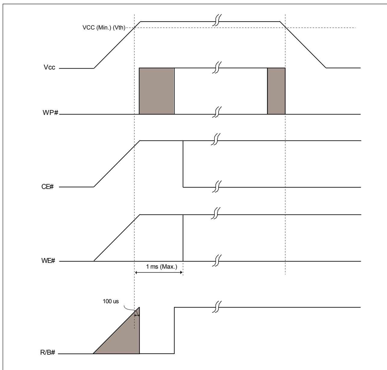
Figure 39. Power On/Off Sequence
