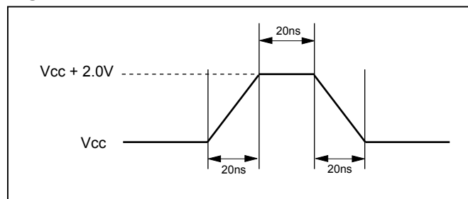
Figure 37. Maximum Positive Overshoot
