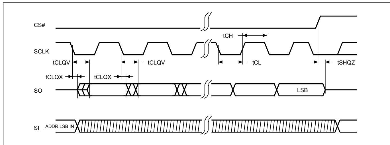
Figure 16. Output Timing
