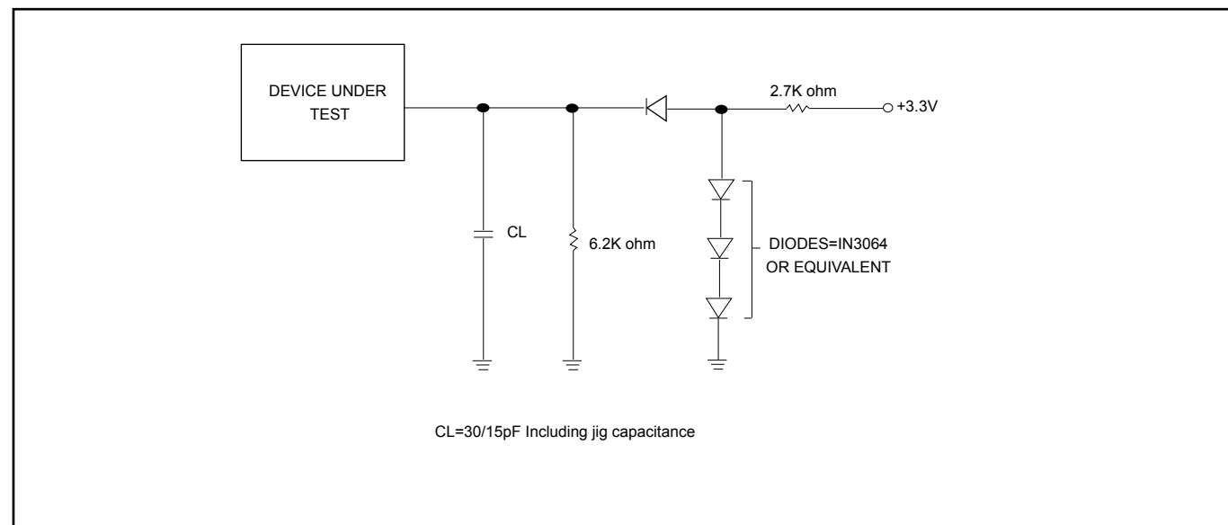
Figure 6. OUTPUT LOADING
