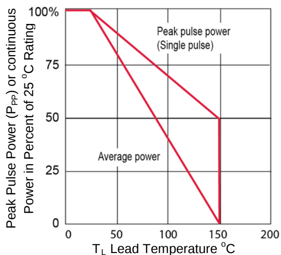
FIGURE 3 Derating Curve
