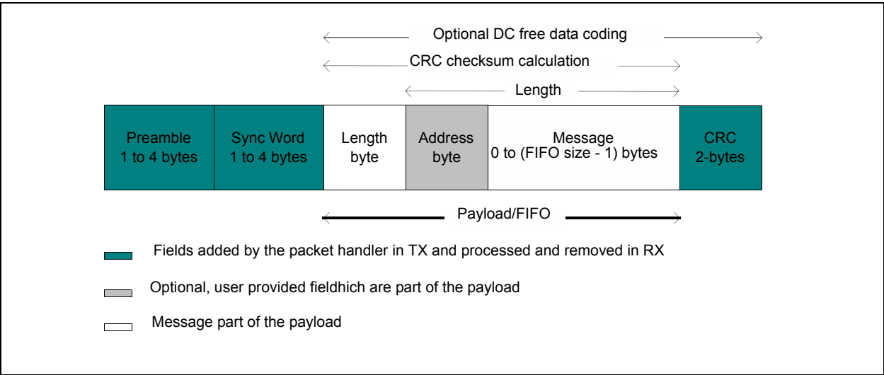
FIGURE 3-27: VARIABLE LENGTH PACKET FORMAT
