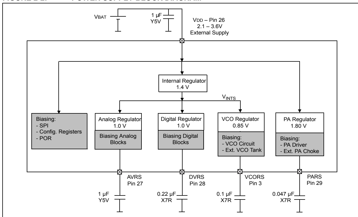
FIGURE 2-2: POWER SUPPLY BLOCK DIAGRAM
