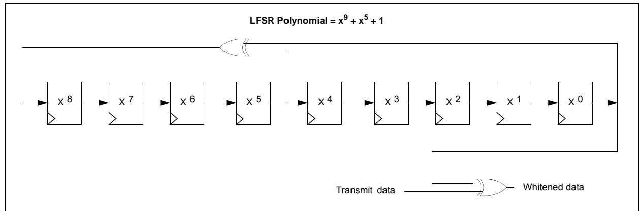
FIGURE 3-31: DATA WHITENING
