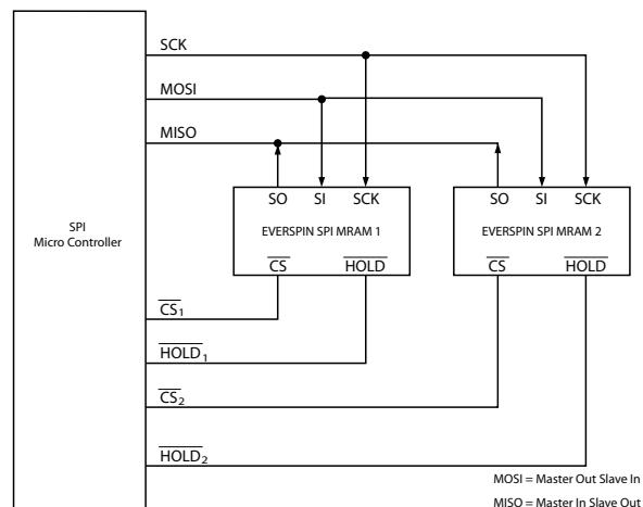
Figure 2 – System Configuration
