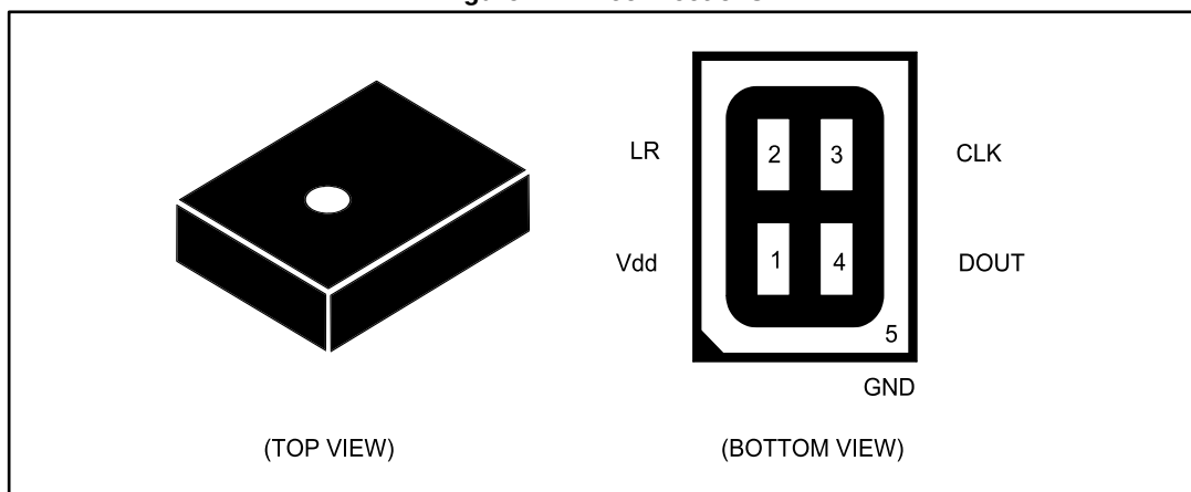
Figure 1: Pin connections
