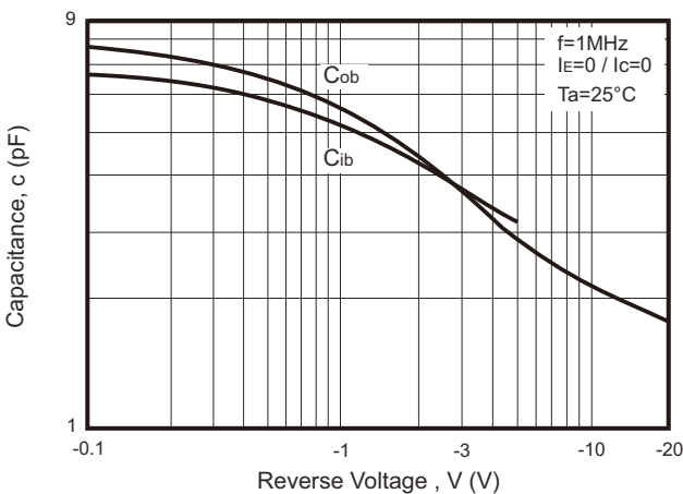
Fig. 6 - C_{ob}/C_{ib} - V_{CB}/V_{EB}
