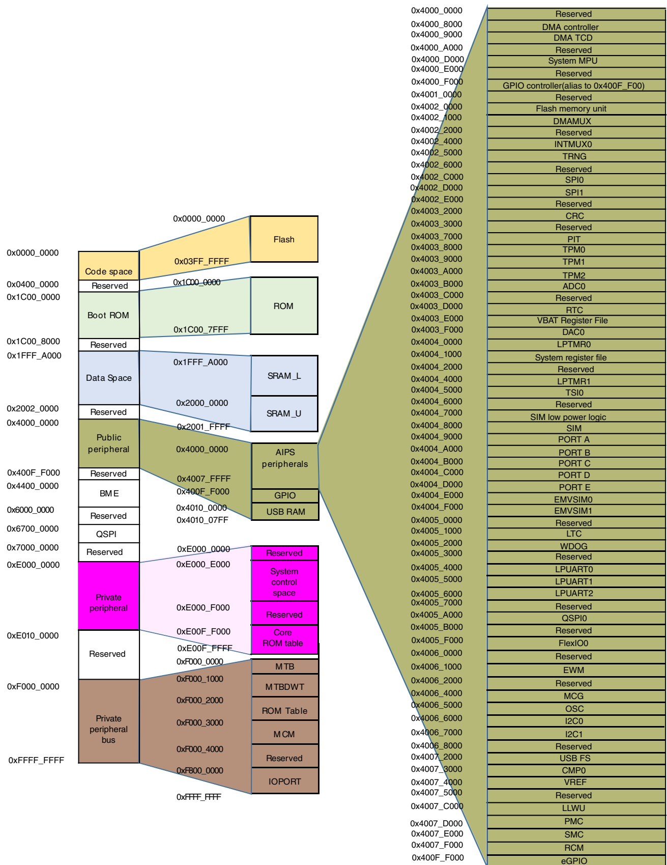
Figure 4. Memory map
