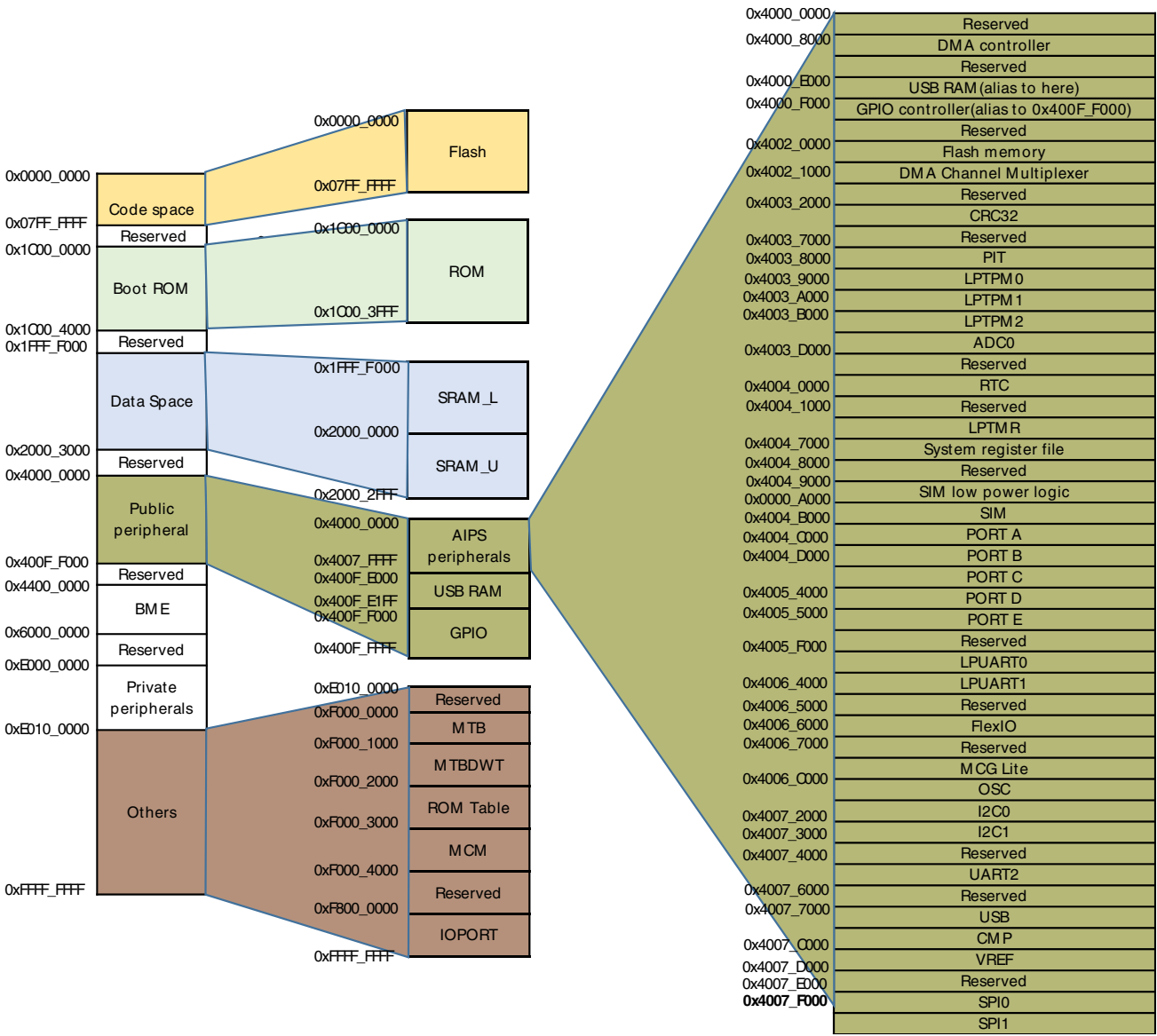
Figure 5. Memory map
