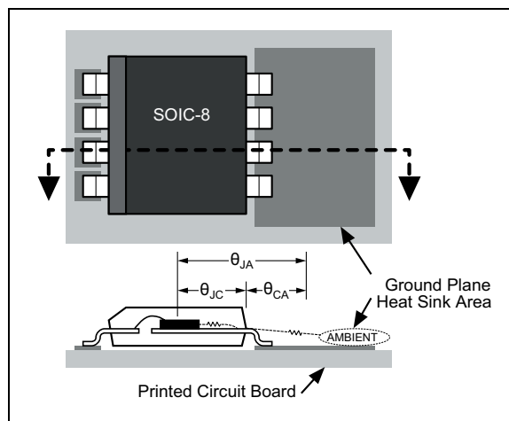
FIGURE 5-11: Thermal Resistance.
