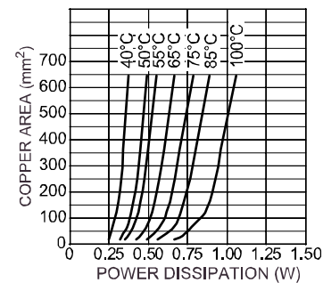
Figure 4. Copper Area vs. Power-MSOP Power Dissipation ( \Delta T_{JA} )
