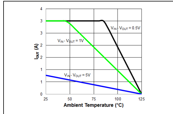
FIGURE 2-42: MIC2930x I_{OUT} vs. T_A SOA (TO-263).
