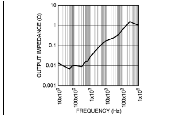
FIGURE 2-40: MIC2930x Output Impedance vs. Frequency.
