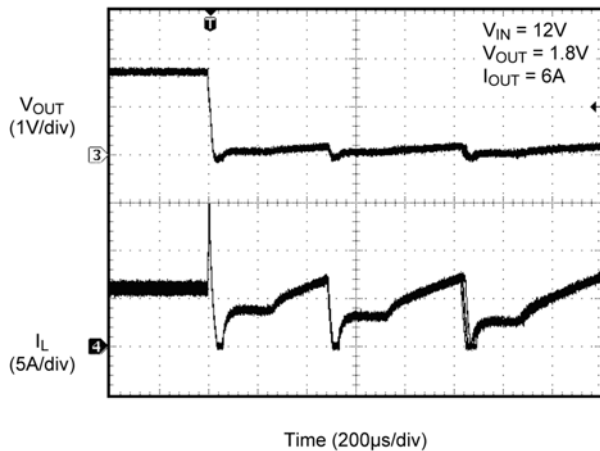
Short Circuit
