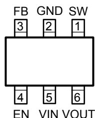
6- Pin Thin SOT-23 (D6)
