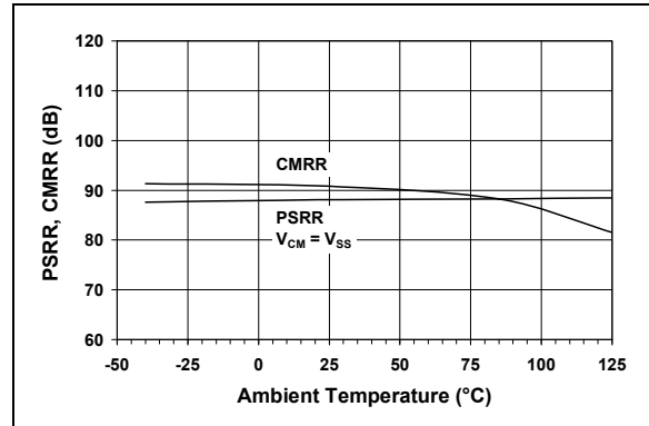
FIGURE 2-11: CMRR, PSRR vs. Ambient Temperature.
