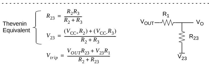
EXAMPLE 6-2: SINGLE-SUPPLY “WINDOW” DAC.
