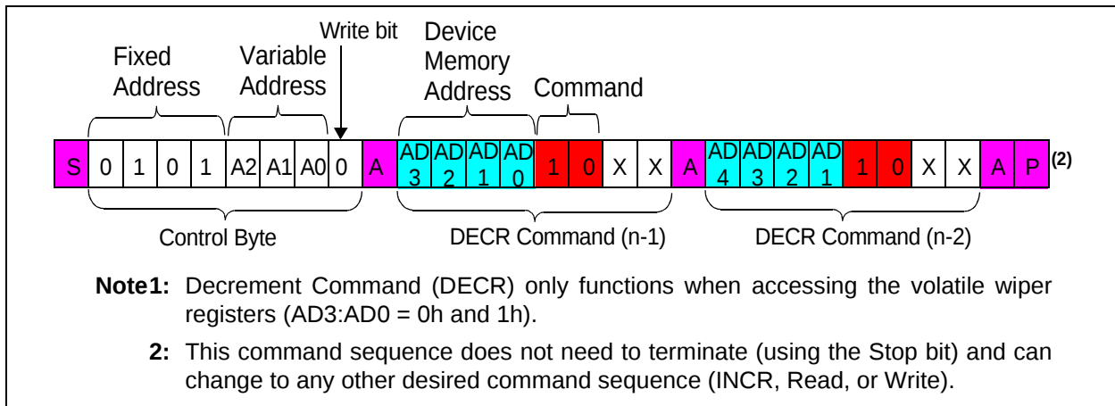
FIGURE 7-8: I²C Decrement Command Sequence.
