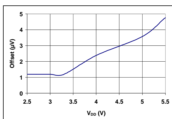
FIGURE 2-11: Offset Error vs V_{DD} ( V_{CM} = 0\text{V} ).
