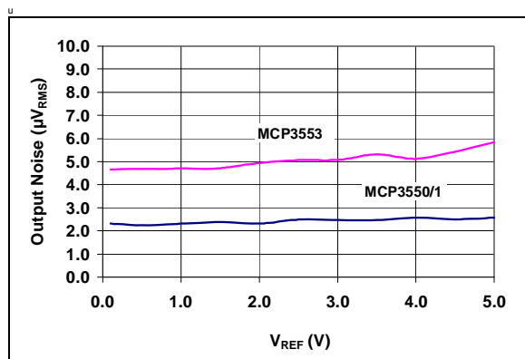
FIGURE 2-8: Output Noise vs. V_{REF} .
