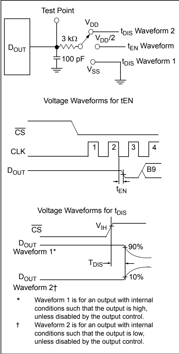
FIGURE 1-3: Load circuit for t DIS and t EN .
