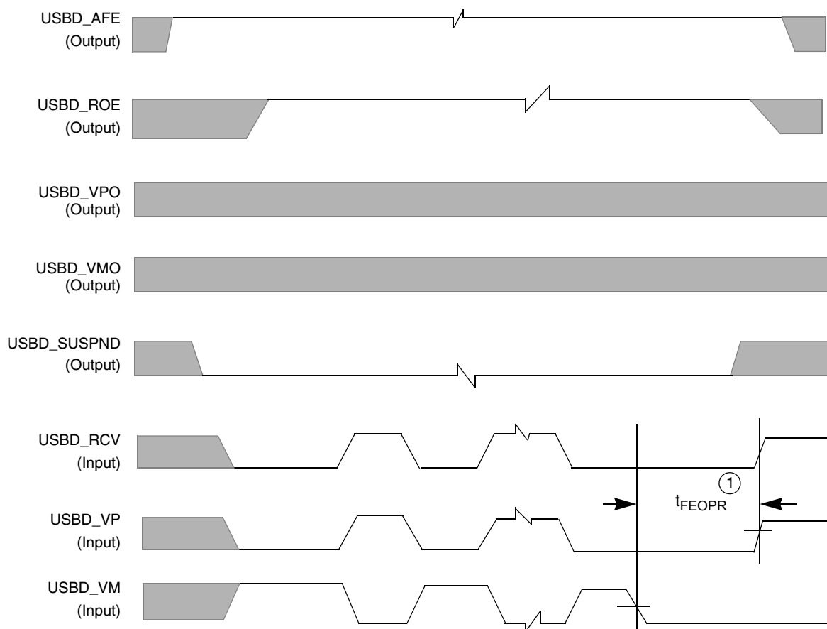
Figure 48. USB Device Timing Diagram for Data Transfer from USB Transceiver (RX)
