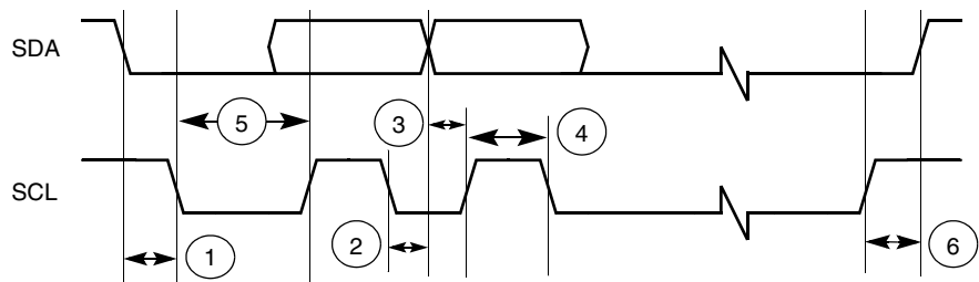
Figure 49. Definition of Bus Timing for I²C
