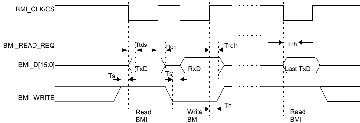
Figure 10. Memory Interface Slave Mode, External Bus Master Read/Write to BMI Timing (MMD_MODE_SEL=0, MASTER_MODE_SEL=0)
