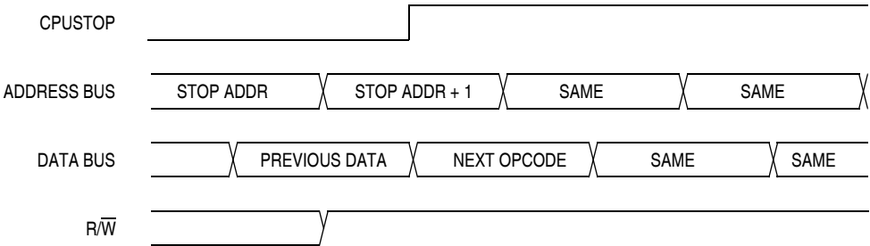
Figure 13-17. Stop Mode Entry Timing
