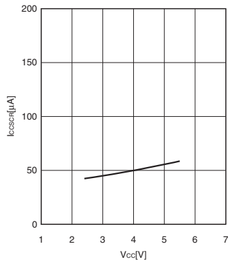
I_{CCSCR} - V_{CC} T_A = +25^{\circ}\text{C} , F_{MPL} = 50 \text{ kHz} (divided by 2) Sub-CR clock mode
