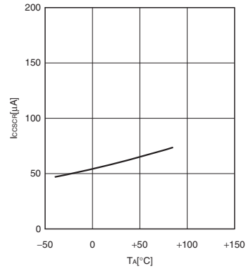
I_{CCSCR} - T_A V_{CC} = 5.5 \text{ V} , F_{MPL} = 50 \text{ kHz} (divided by 2) Sub-CR clock mode
