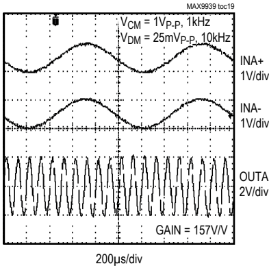
COMMON-MODE REJECTION RESPONSE
