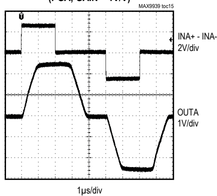
RECOVERY FROM INPUT OVERLOAD (PGA, GAIN = 1V/V)
