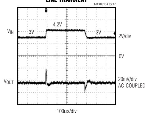
LINE TRANSIENT
