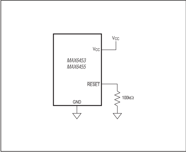
Figure 6. Ensuring \overline{\text{RESET}} Valid to V_{CC} = 0
