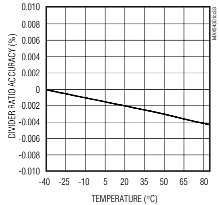
MAX543_B DIVIDER RATIO ACCURACY vs. TEMPERATURE (RATIO = 2)
