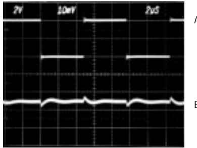
DIGITAL FEEDTHROUGH
