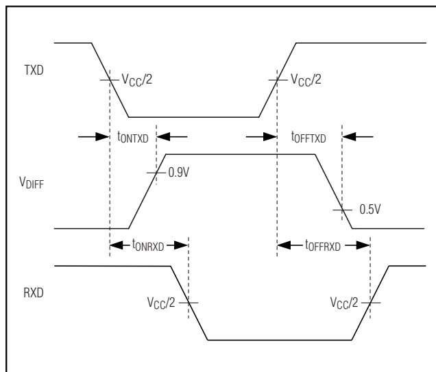
Figure 1. Timing Diagram
