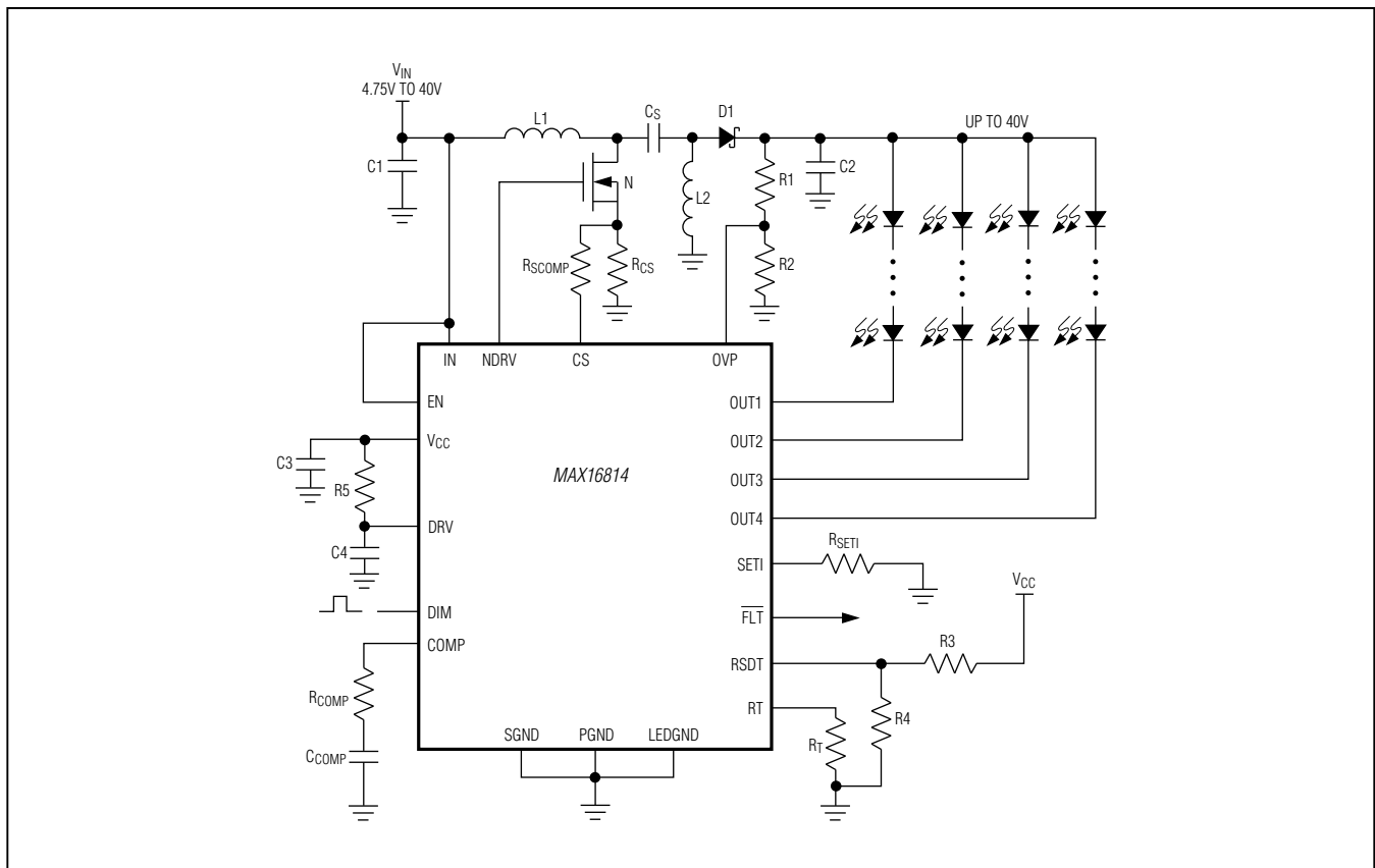
Figure 5. SEPIC Configuration
