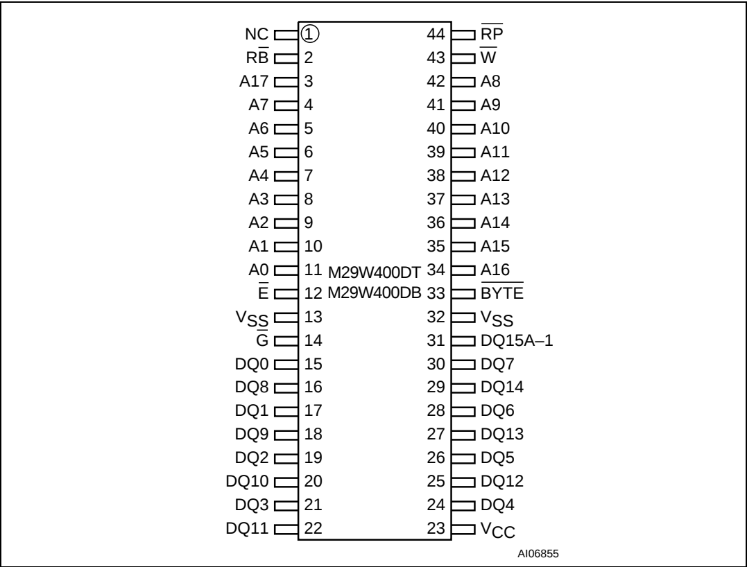
Figure 2. SO connections
