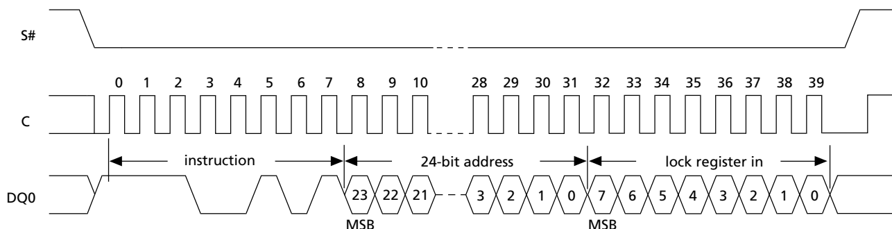
Figure 19: WRITE to LOCK REGISTER Instruction Sequence
