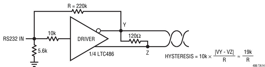
RS232 to RS485 Level Translator with Hysteresis
