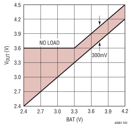
Figure 2. V_{\text{OUT}} vs BAT
