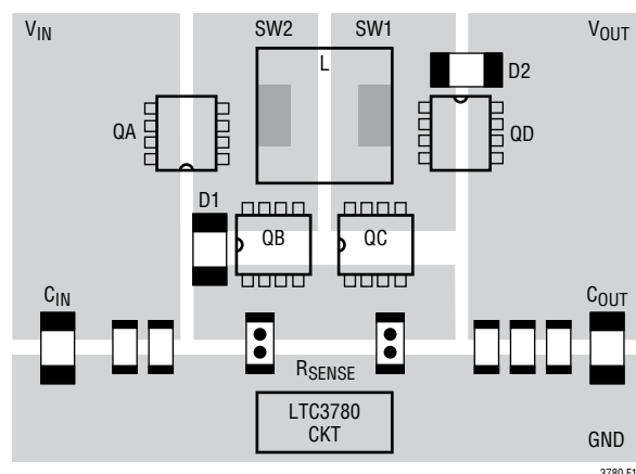
Figure 10. Switches Layout
