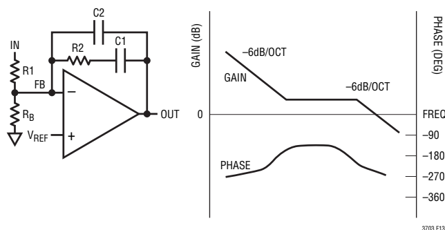
Figure 13. Type 2 Schematic and Transfer Function
