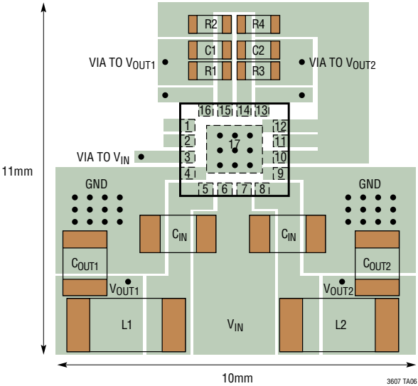
1mm Height, 1.8V/3.3V Buck Regulator Using Chip Inductors
