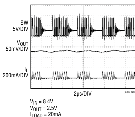
Pulse-Skipping Mode
