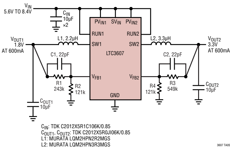
1mm Height, 1.8V/3.3V Buck Regulator Using Chip Inductors
